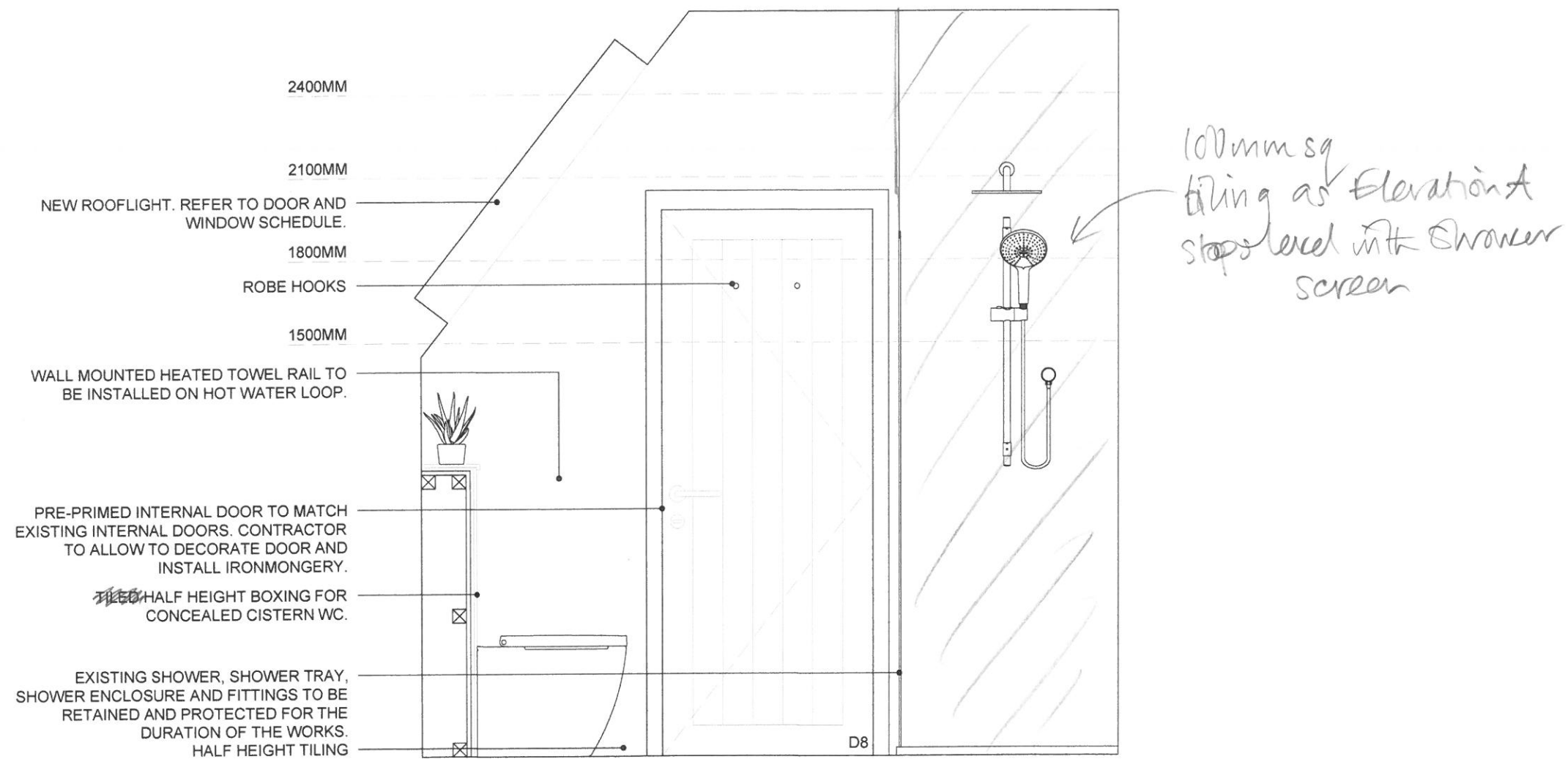
GUEST BEDROOM 01 ENSUITE ELEVATION D
