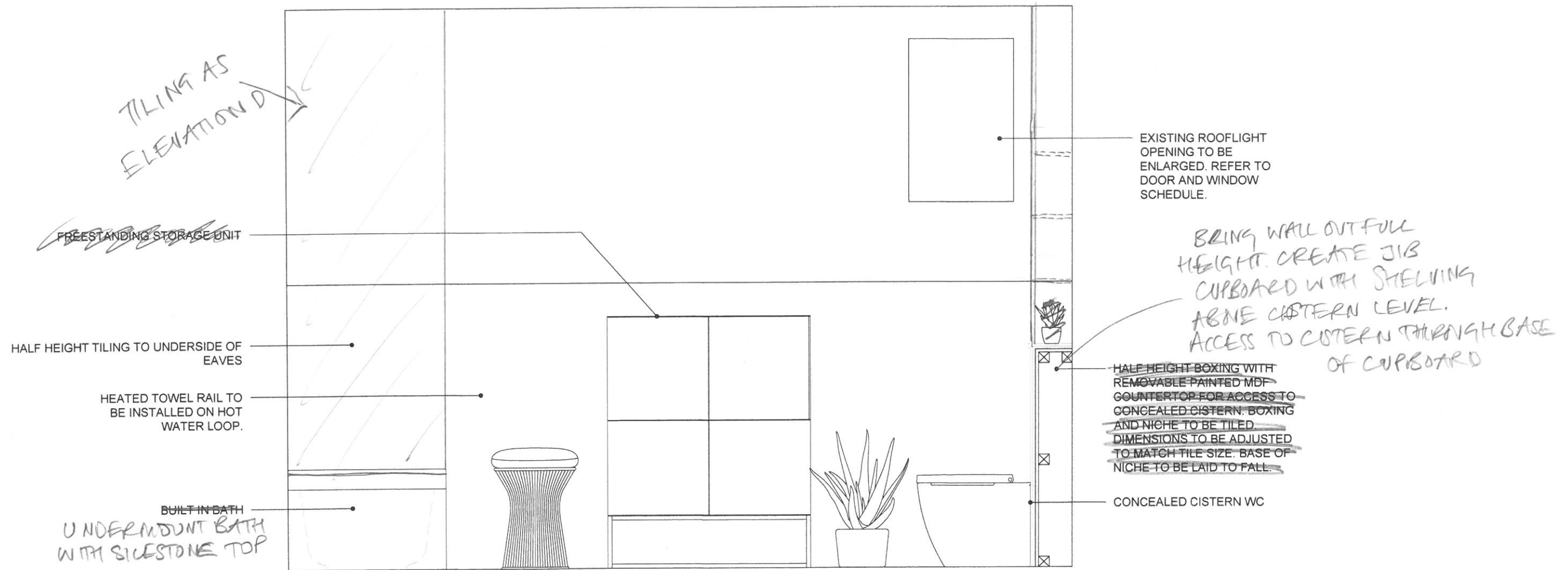
FAMILY BATHROOM ELEVATION A
