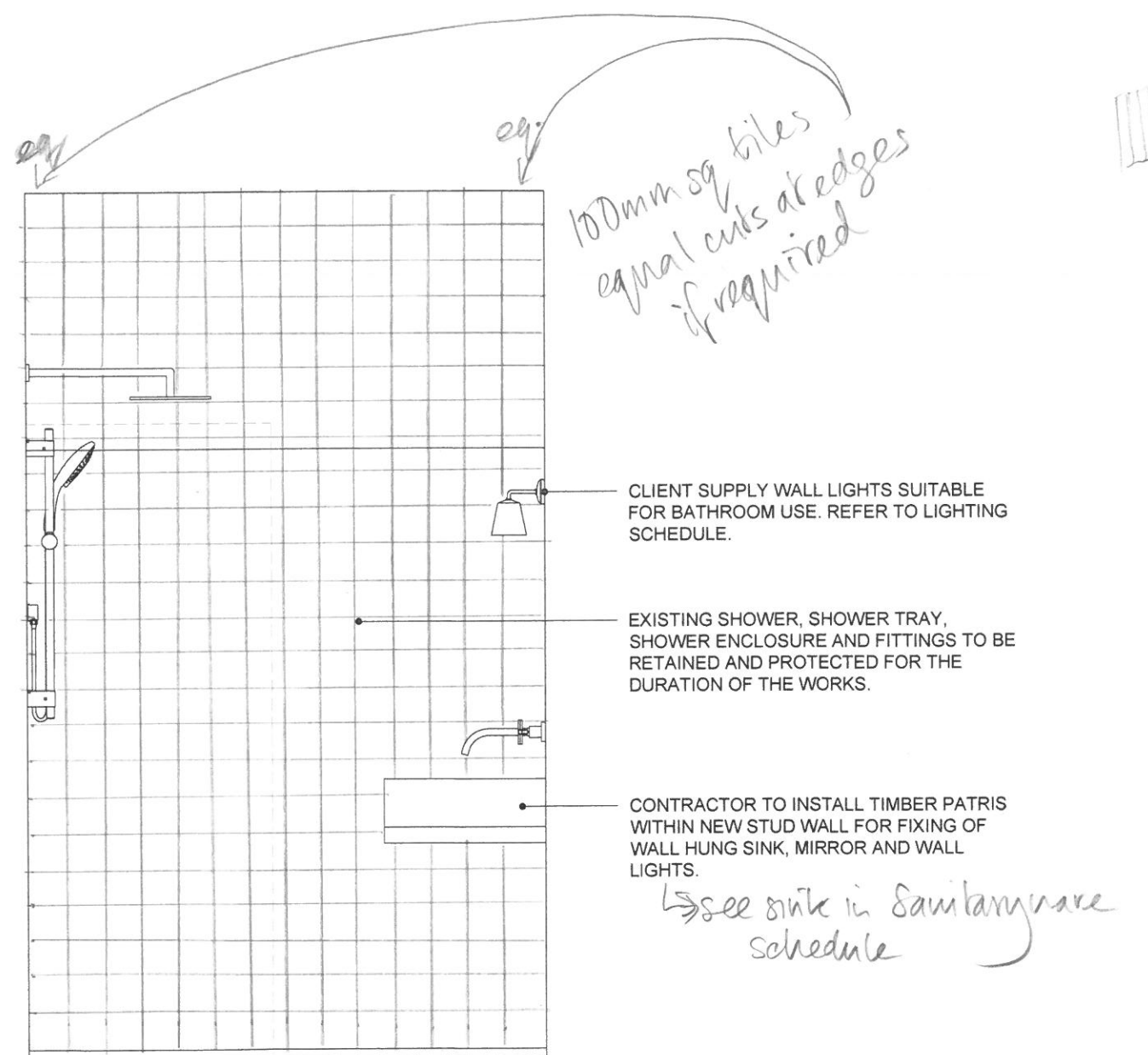
GUEST BEDROOM 01 ENSUITE ELEVATION A
