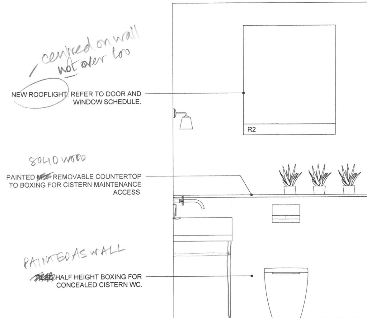
GUEST BEDROOM 01 ENSUITE ELEVATION C
