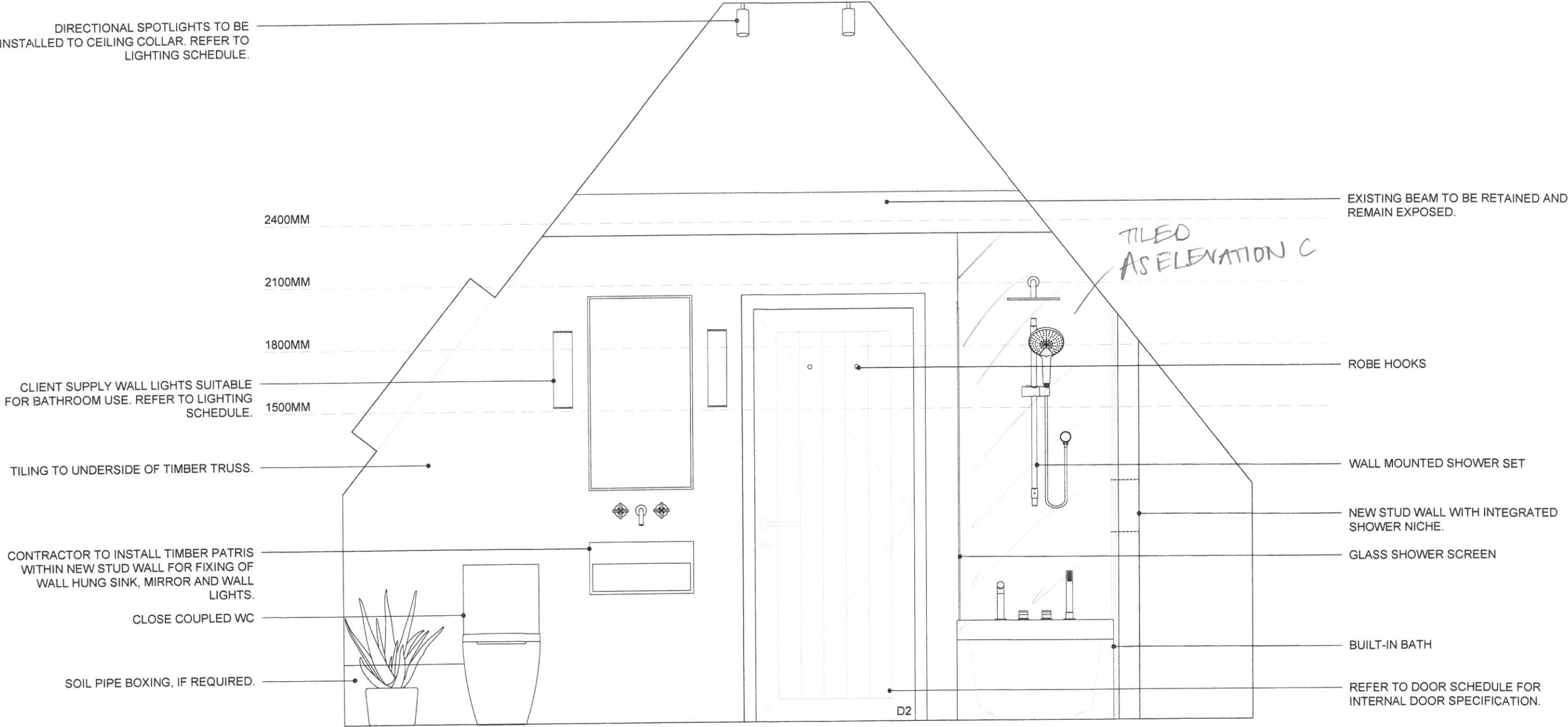
GUEST BEDROOM 02 ENSUITE ELEVATION B
