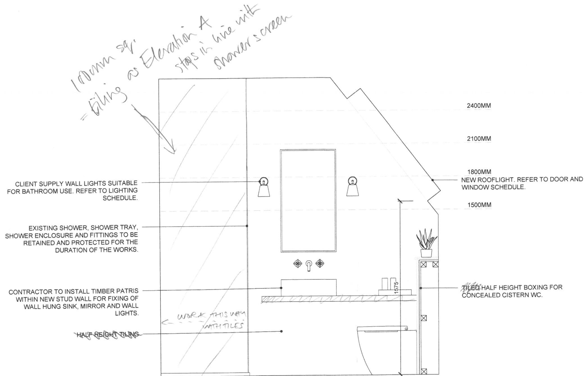
GUEST BEDROOM 01 ENSUITE ELEVATION B
