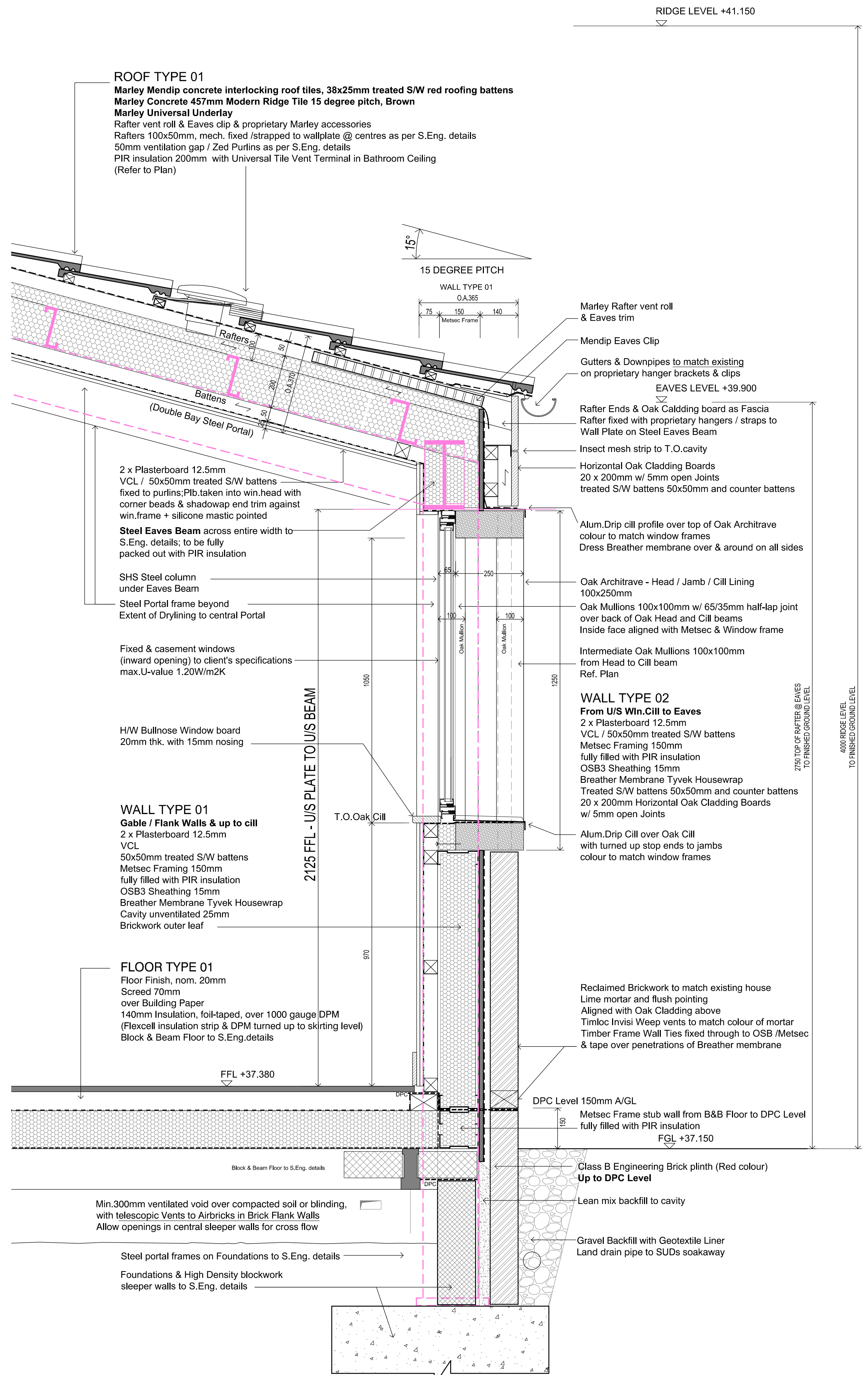
Detail Section 2 (Floor / Wall / Window Cill & Head / Eaves)
