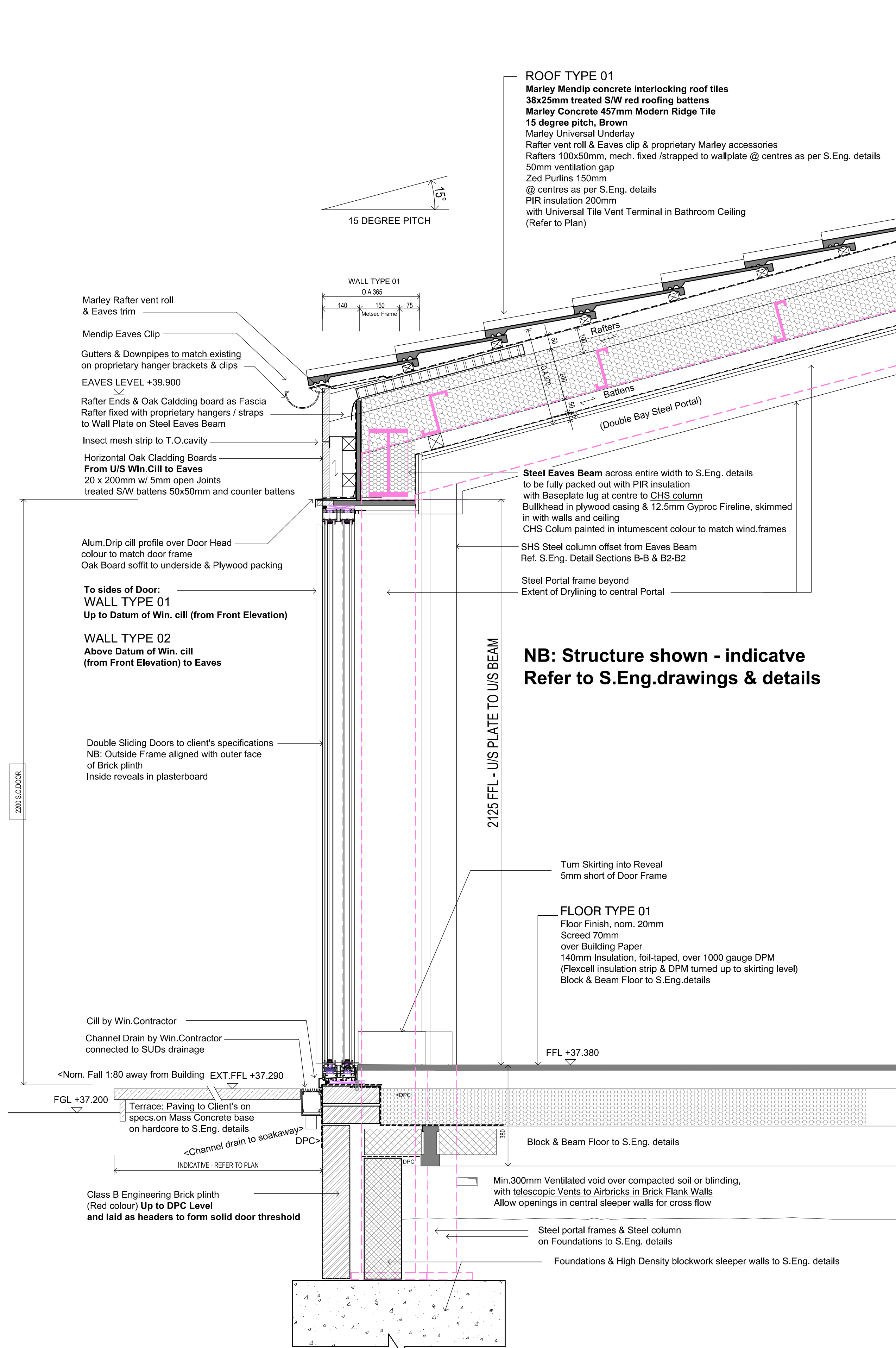
Detail Section 1 (Floor / Wall / Sliding Door Threshold & Head / Eaves)
