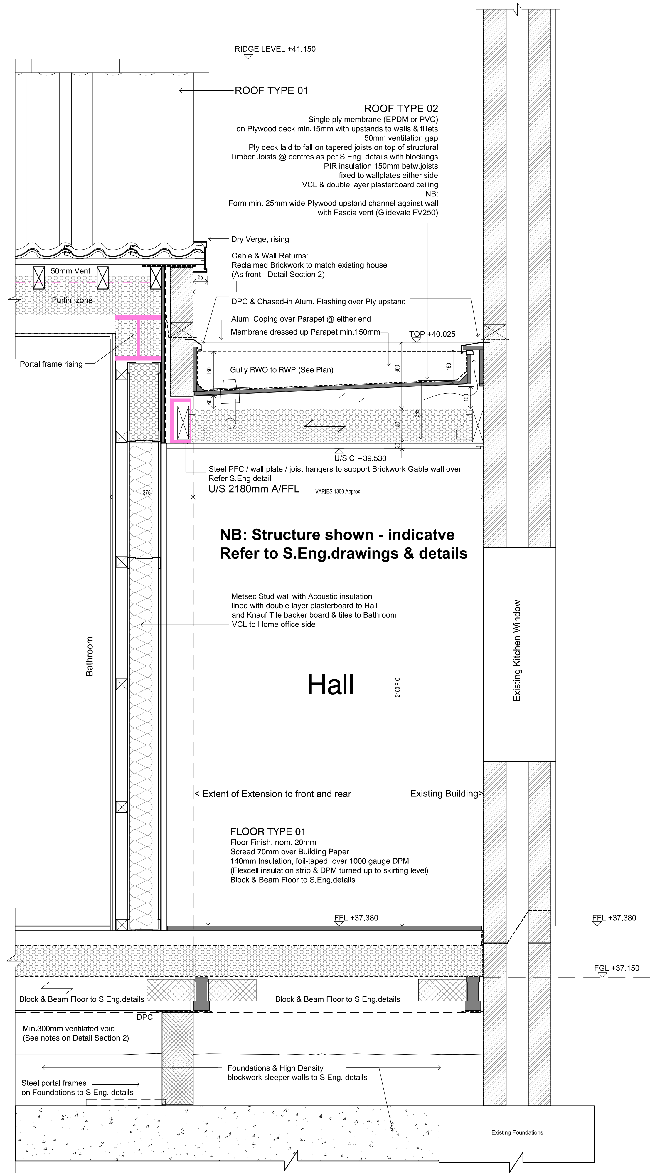
Detail Section 3 (Hall Floor / Roof / Wall Abutment)
